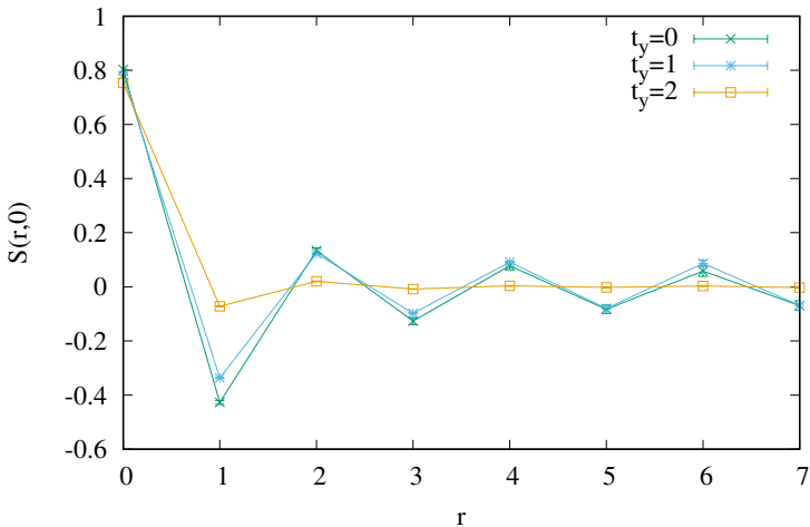
L=14 Hubbard Ladder, \beta t=10 , U/t=4
